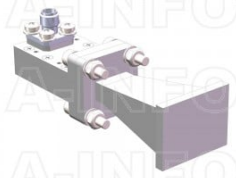
LB-42-10-C-SFSPO Standard Gain Horn Antenna 18-26.5GHz 10dB Gain SMA Female
