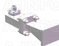
LB-42-10-C-3.5FSP Standard Gain Horn Antenna 18-26.5GHz 10dB Gain 3.5mm Female
